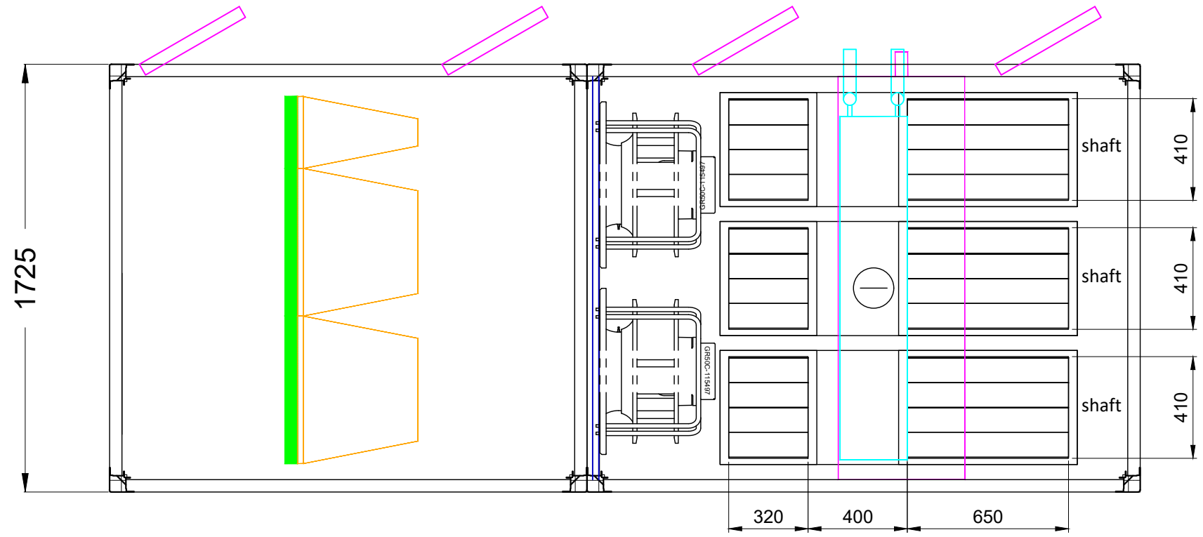
Top View
